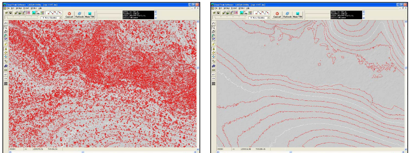
Figure 4-3. Unfiltered (left) and bare-earth (right) contour data sets of the same area
