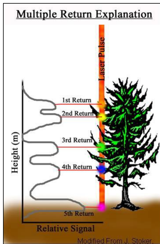
Figure 5-1. Multiple returns from single laser pulse
