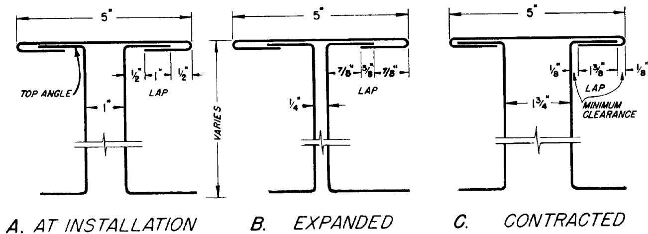
Figure 39. Movement of expansion joints.
