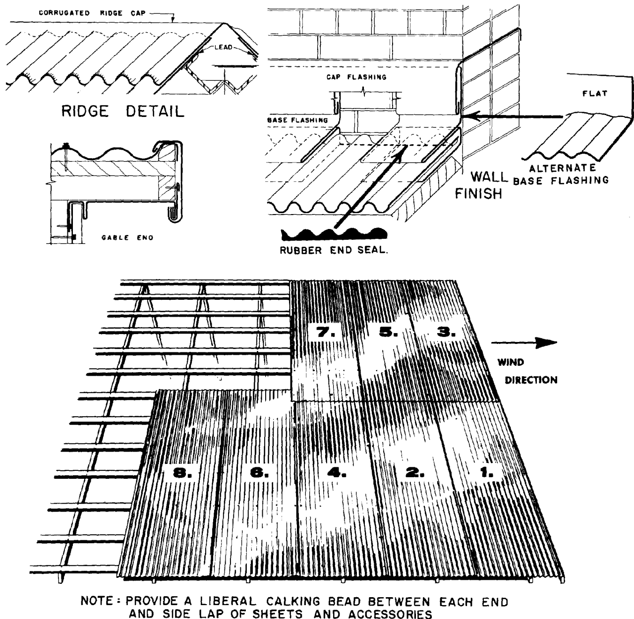
Figure 46. Corrugated roofing.
