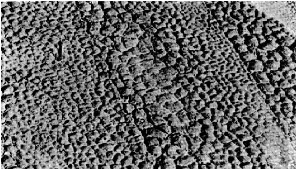
Figure 17. Alligatoring and cracking of a cold coating over alligatoring asphalt surface after 1 year exposure.
