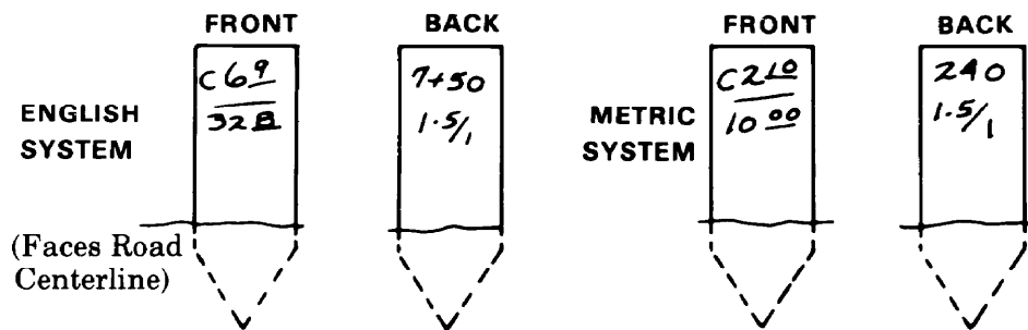
Figure 2-3. Marking slope stakes
