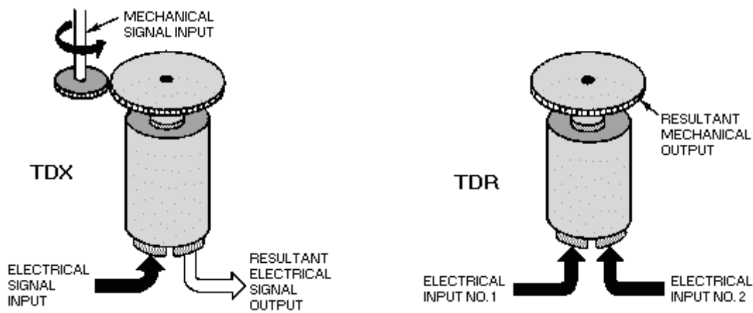
Figure 1-18.—Torque differentials.
