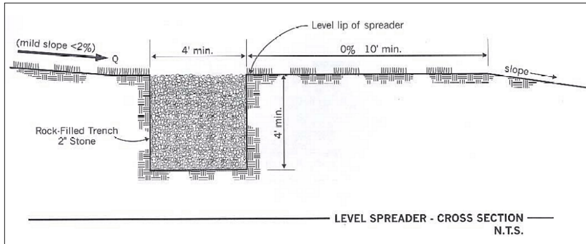
FIGURE 5. LEVEL SPREADER
