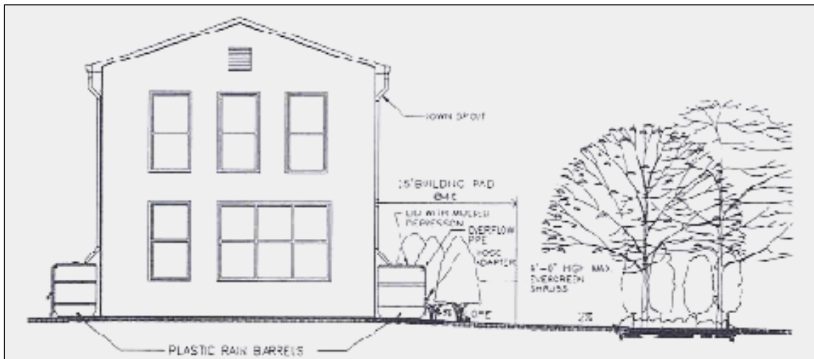
FIGURE 9. RAIN BARRELS
