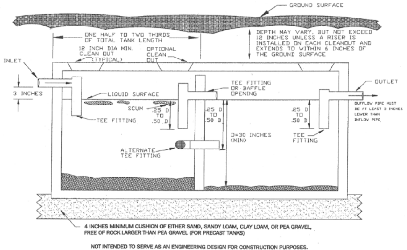
(6) Figure 6. Two Compartment Septic Tank.
