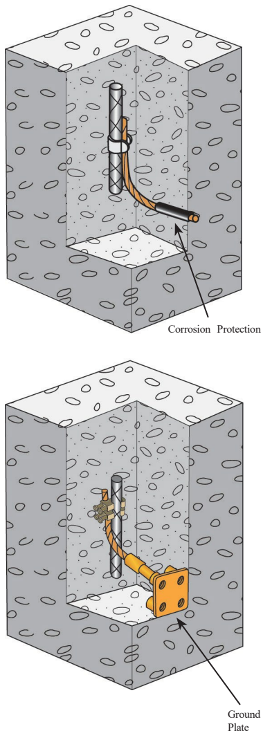
Figure 24. Ground plates are convenient and eliminate the need for corrosion protection.
