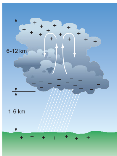
Figure 2. Typical charge distribution in cumulonimbus cloud.
