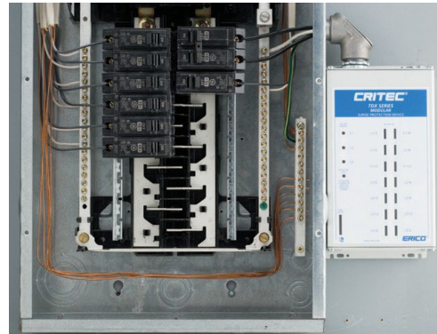
(a) External mounting SPDs.
