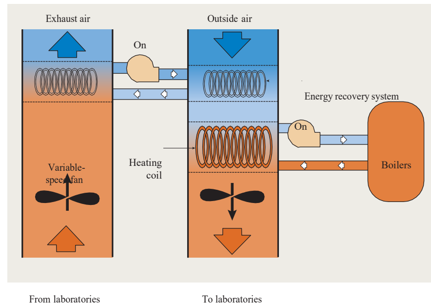
Air-to-air sensible energy recovery system using run-around coils.
