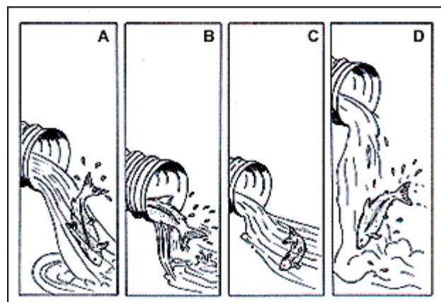
Figure 21. Improperly installed culverts can block fish passage: (A) water velocity too great, (B) water in culvert too shallow, (C) no resting pool below culvert,
