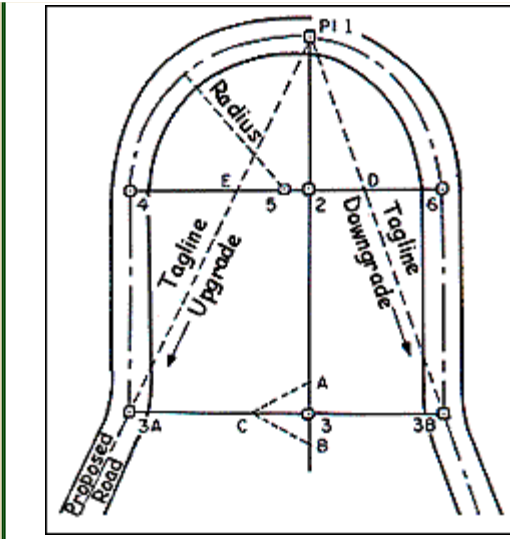
Figure 4. A switchback is needed when a straight road would exceed maximum acceptable grade. (Redrawn and adapted from Figure 2.4-3, Darrach et al. 1981)
