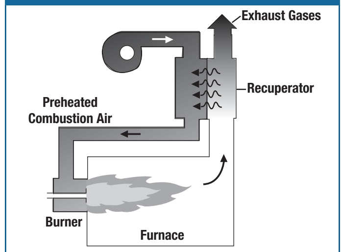
Figure 11. Recuperator system for preheating combustion air losses.
