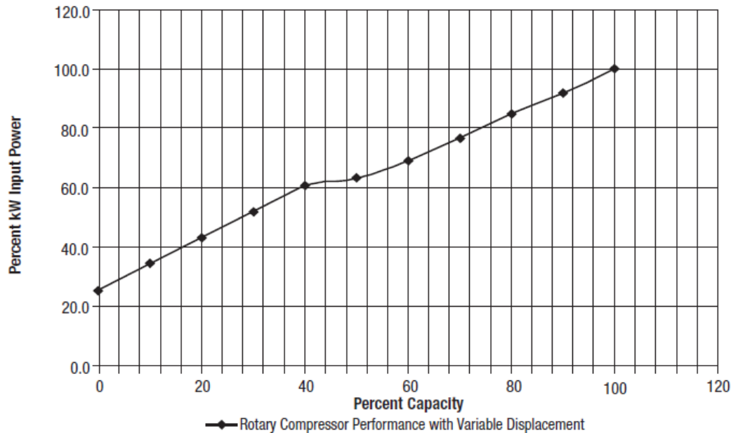
Figure 2.7 Lubricant-Injected Rotary Compressor Performance with Variable Displacement.
