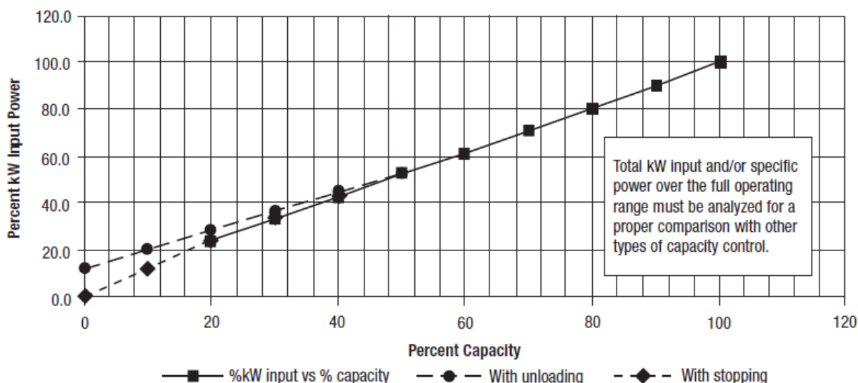
Figure 2.8 Lubricant-Injected Rotary Compressor Performance with Variable Speed Control.
