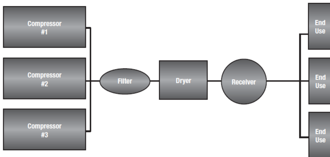
Figure 2.2 Compressed Air System Block Diagram.
