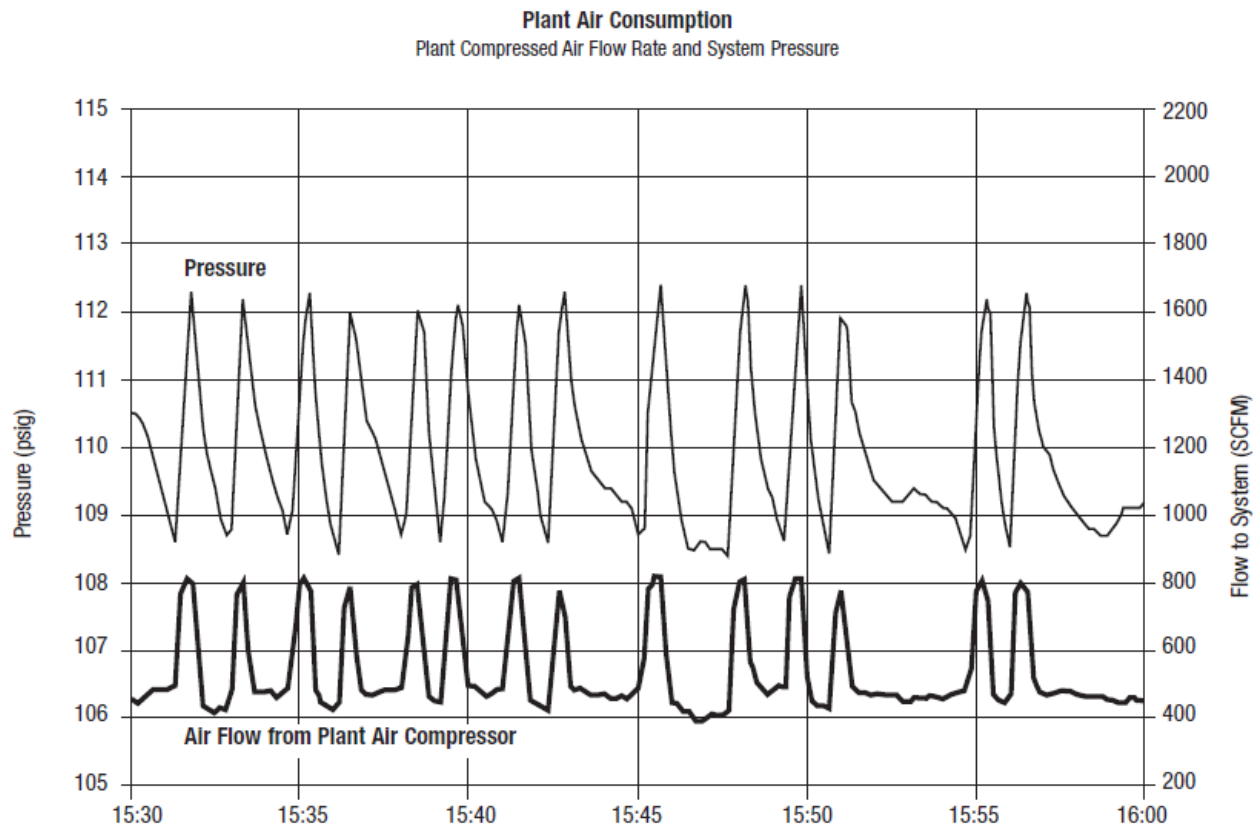
Figure 2.4 Pressure Profile Over a Defined Time Period.
