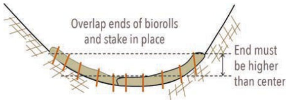
Figure 21: Proper check dam installation
