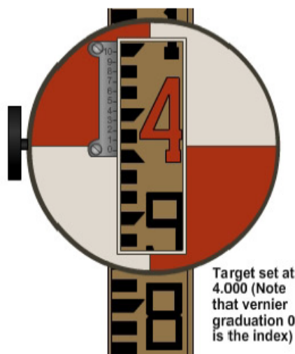
Figure 23 – Target.
