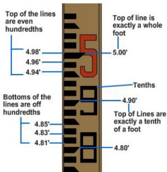
Figure 5-21 – Philadelphia rod marking
