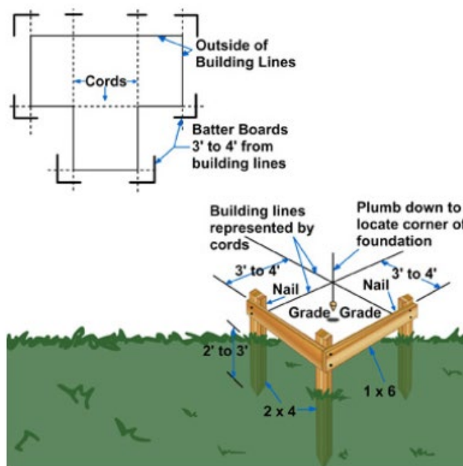
Figure 28 – Batter boards.
