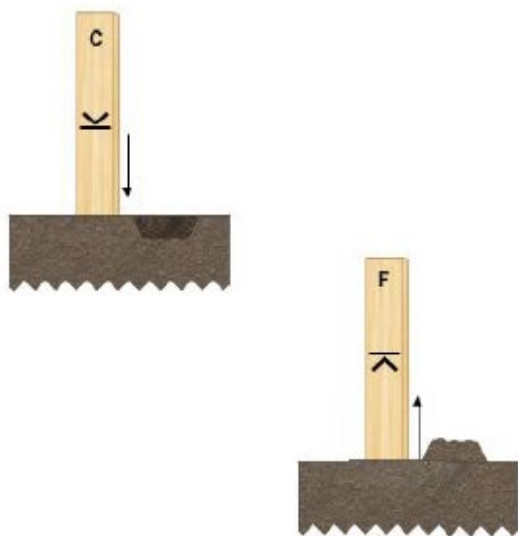
Figure 36 – Cut and fill crowfoot symbol.
