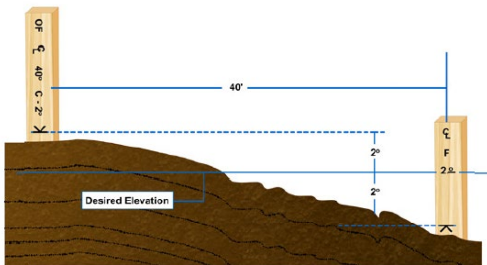
Figure 41 – Difference in elevation between the offset stake crowfoot and desired grade at center stake.
