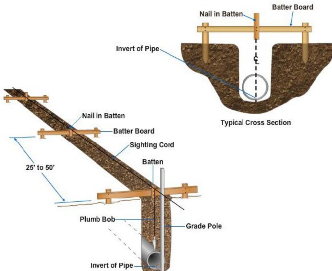
Figure 29 – Use of batter boards (with batters) for utility stakeout.
