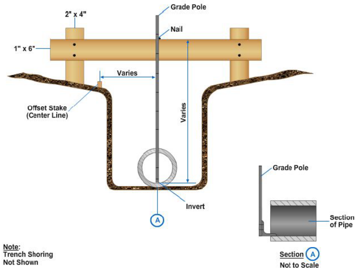
Figure 30 – Batter boards (without battens) for utility stakeout.
