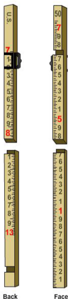
Figure 19 – Back and face of Philadelphia leveling rod.
