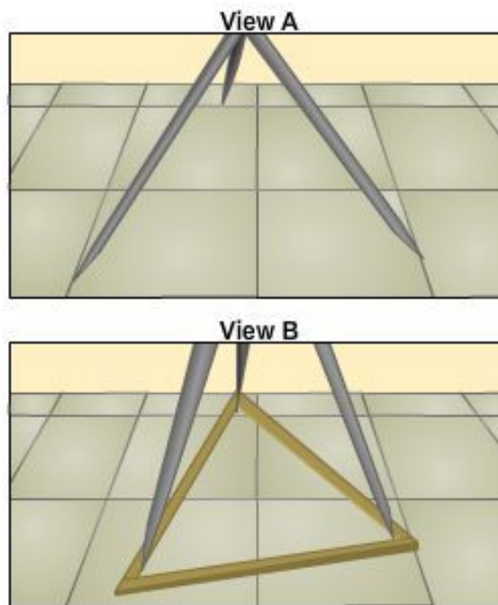
Figure 16 – Methods of preventing tripod legs from spreading.
