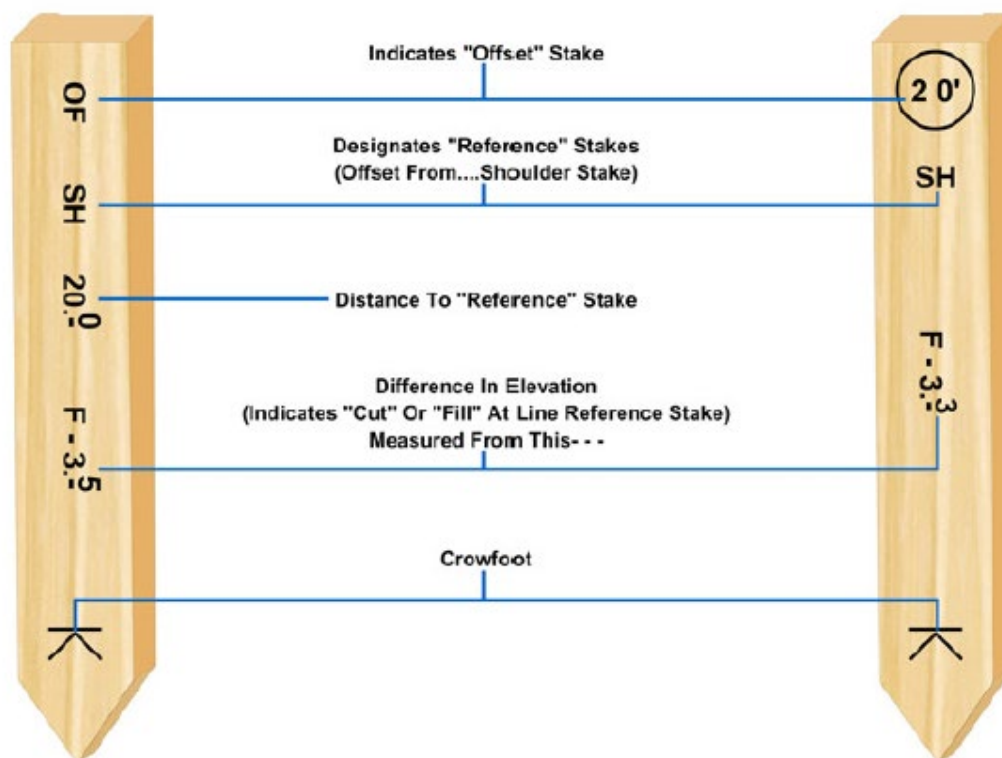
Figure 40 – Reference information found on an offset stake.
