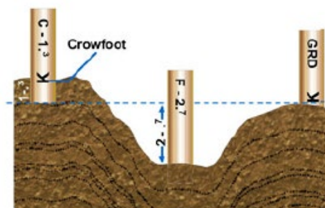
Figure 39 – Cut, fill, and on-grade stakes.
