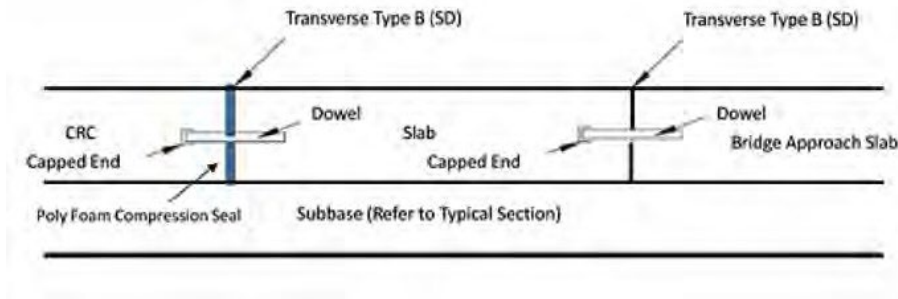
Figure 49. Transition from CRCP using doweled joints.
