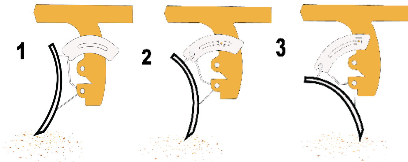
FIGURE 2: Moldboard pitch.
