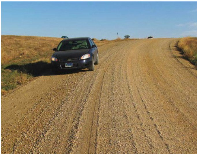
Wrong shape on curve which increases risk of crashes.
