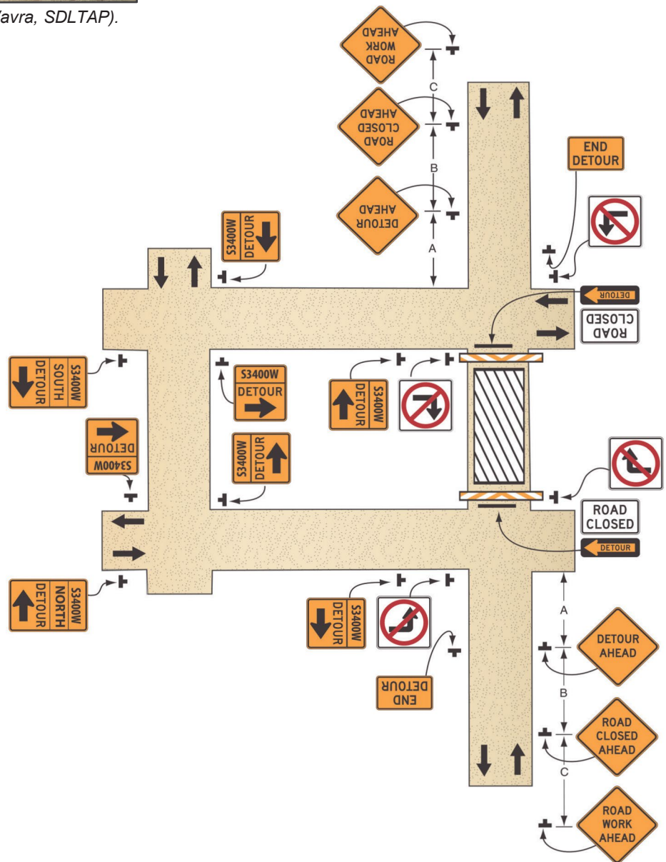
Figure 4. TTC application for reconstruction using a detour.
