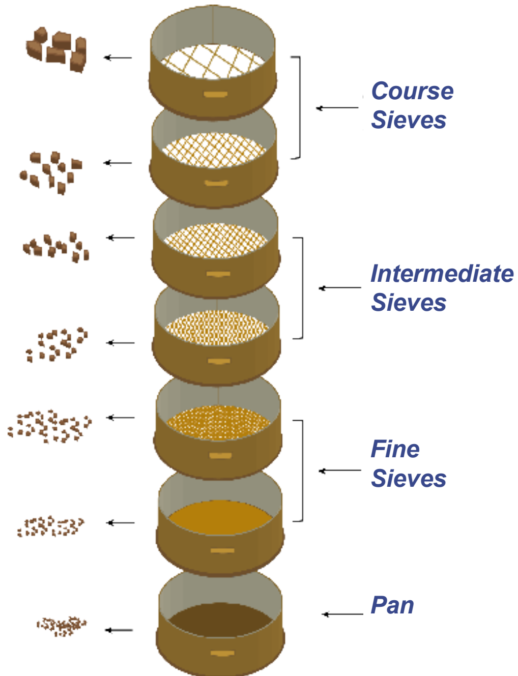
FIGURE 13: Testing gradation. Illustration of stack of sieves used in testing aggregate gradation.
