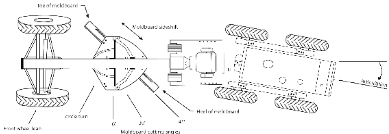
FIGURE 3: Articulated Motorgrader
