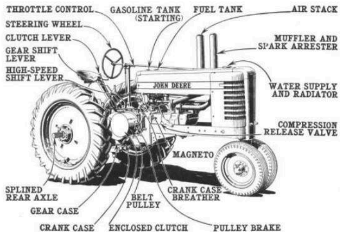
Figure 208—Adjustable tread general-purpose tractor.
