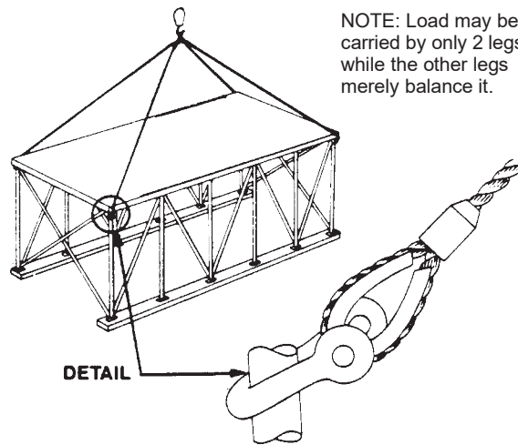
4-LEG BRIDLE HITCH Figure 13
