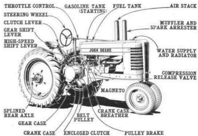
Figure 208—Adjustable tread general-purpose tractor.
