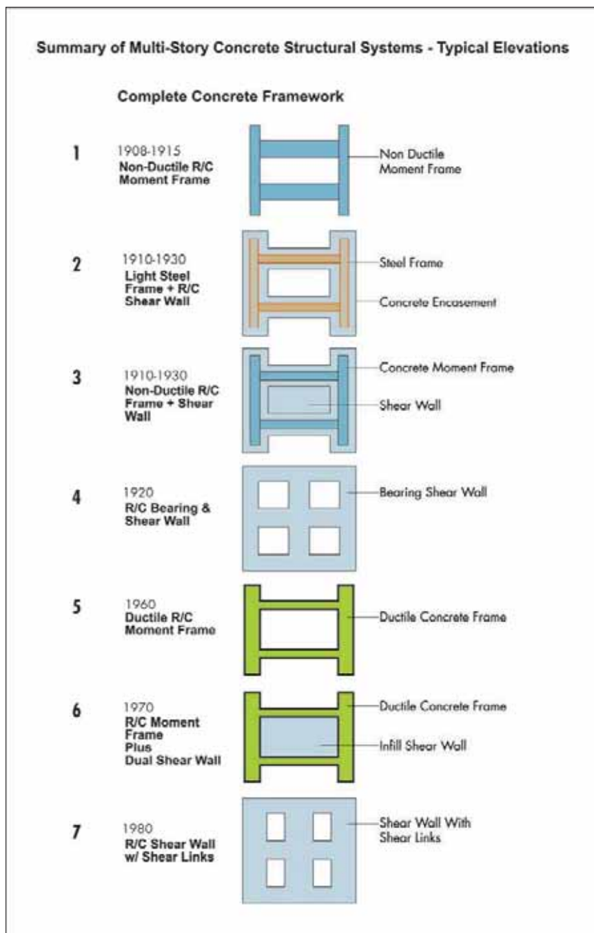
Figure 7-3: Concrete building frameworks
