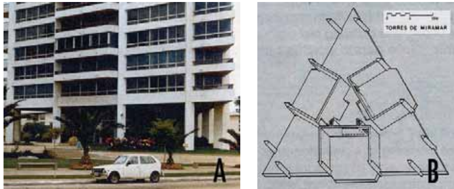
Figure 5-12: This apartment house appears to have a soft first story (Figure 5-12A), but the lateral force-resisting system is a strong internal shear wall box, in which the shear walls act as party walls between the dwelling units (Figure 5-12B). The architect achieved a light and elegant appearance, and the engineer enjoyed an optimum and economical structure.
