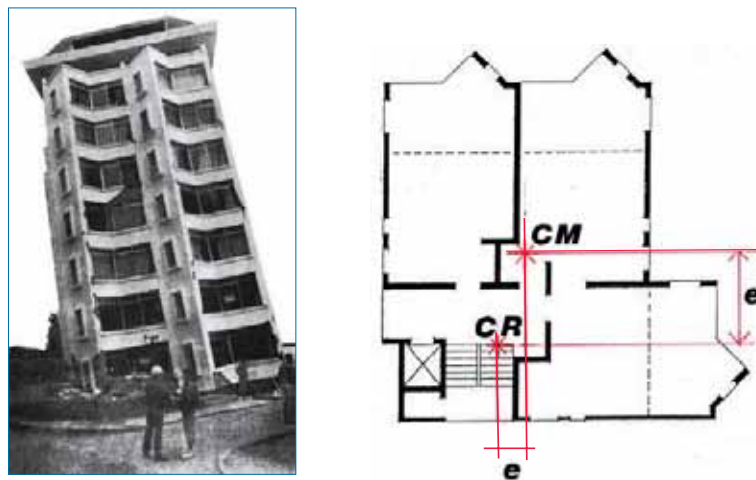
Figure 5-16: Left, the building after the earthquake. Right, typical floor plan showing the Center of Mass (CM), Center of Resistance (CR), and Eccentricity ( e ) along the two axes. PHOTO SOURCE: EERI
