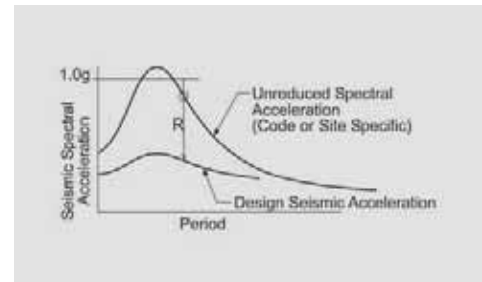
Figure 7-4: Design versus real acceleration.
