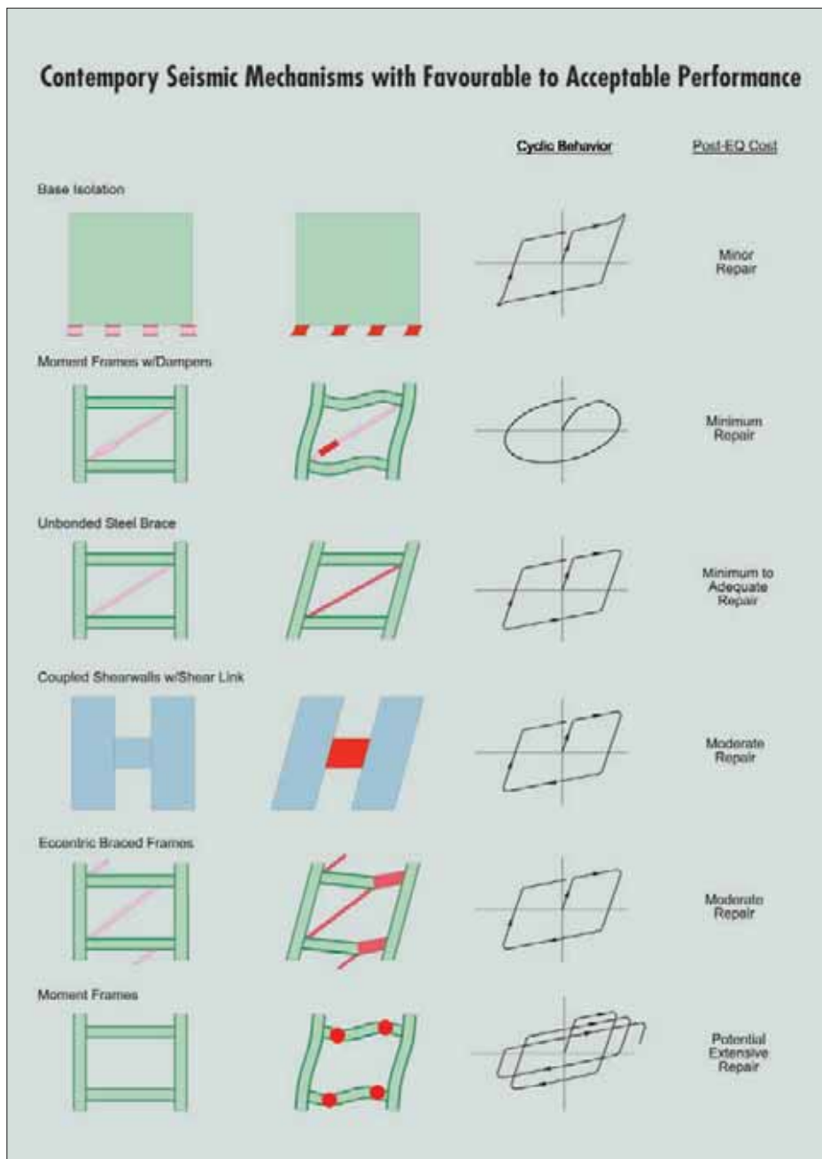
Figure 7-19: Six high-performance seismic structures.
