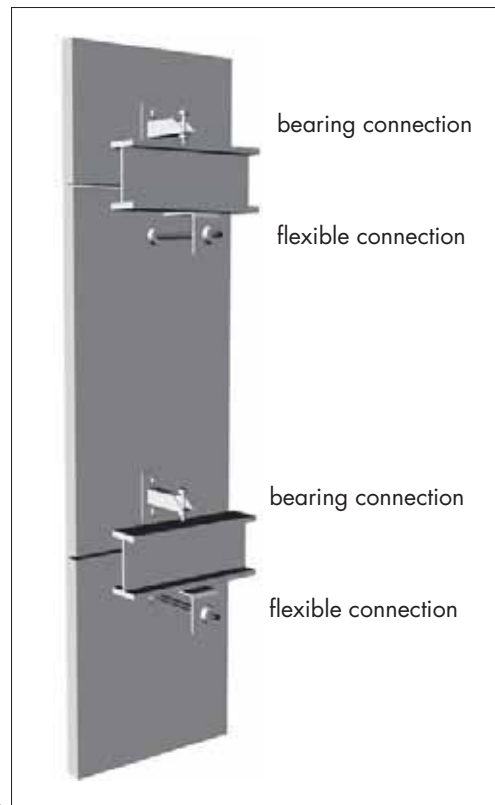
Figure 6-10 Typical floor-to-floor push-pull panel connections. Each beam has a bearing connection at the bottom of a panel and a flexible, or tie-back, connection for the panel below.
