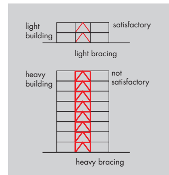
Figure 7-14: Building scale.
