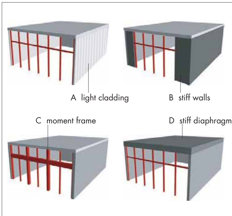
Figure 5-19 Some solutions to store-front type unbalanced-perimeter- resistance conditions
