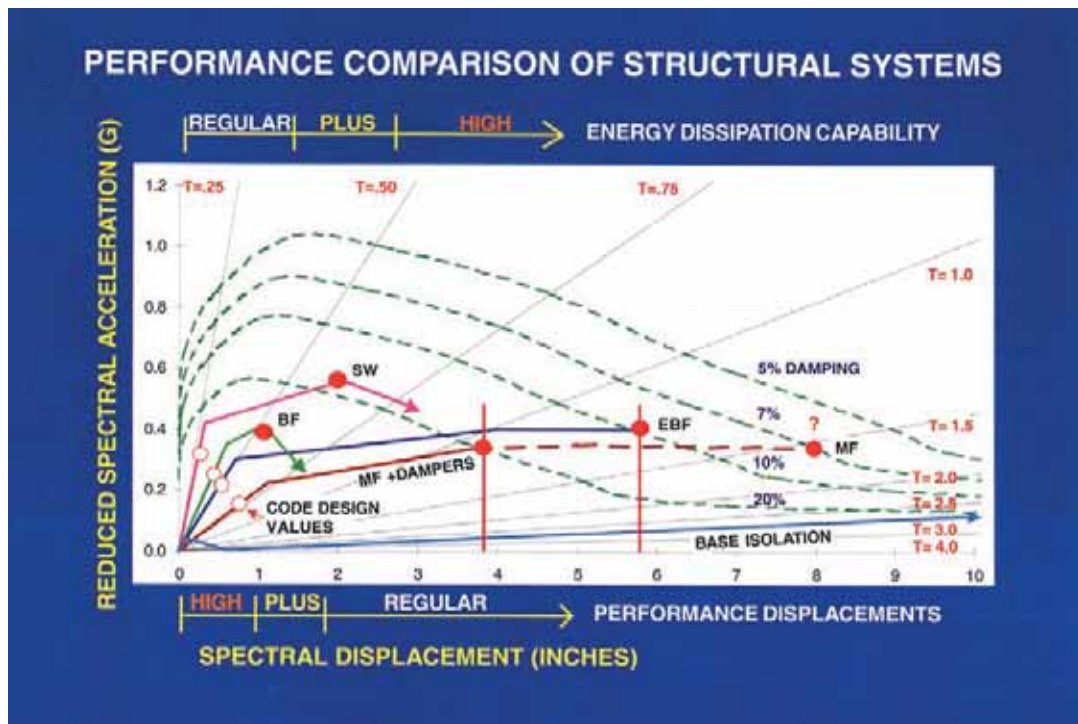
Figure 7-7: Performance characteristics of structural systems.
