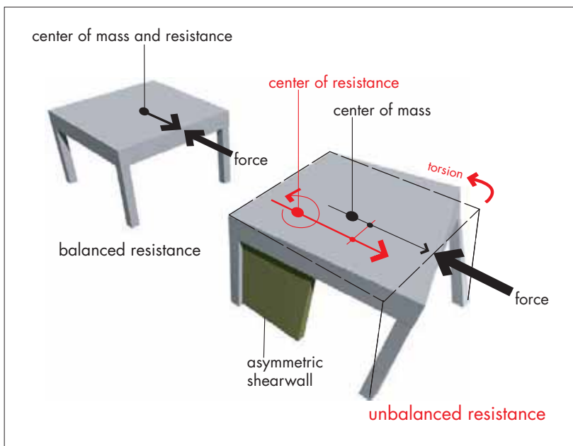
Figure 4-17 Torsional forces.
