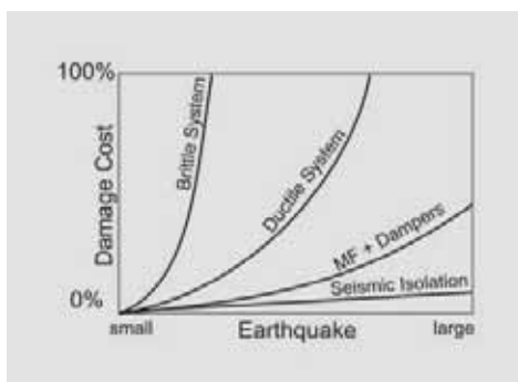
Figure 7-10 System performance.
