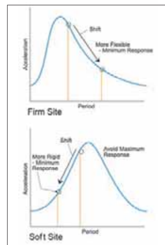
Figure 7-15: Building resonance.
