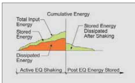
Figure 7-8A: Energy stored.
