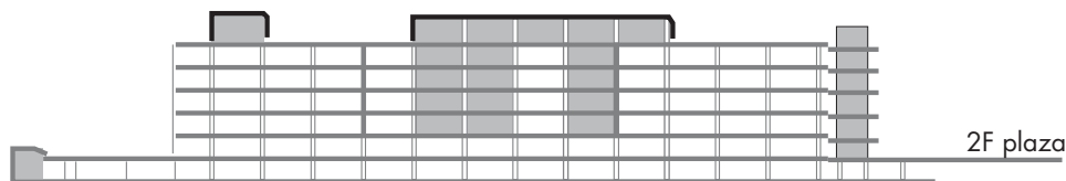
Figure 5-13: Long section, Olive View Hospital. Note that the shear walls stop at the third floor.
