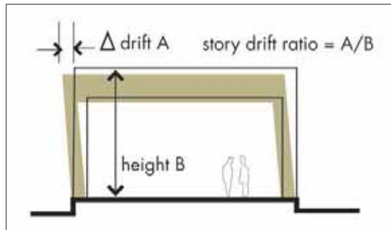
Figure 4-12 Story drift ratio.
