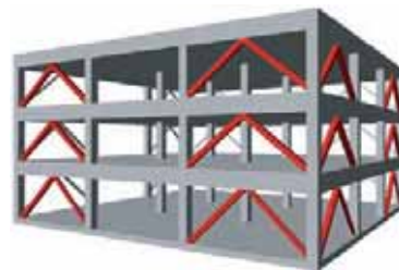
braced frame
