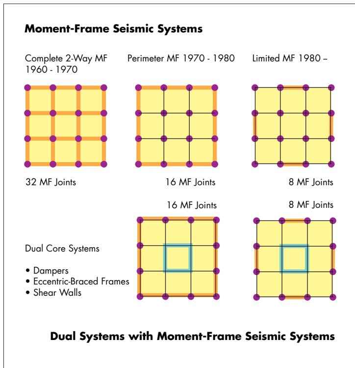
Figure 7-18: Single and multiple system concepts.
