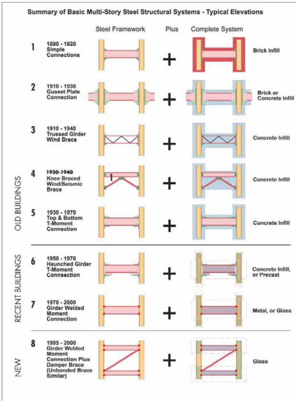
Figure 7-2: Steel building frameworks.
