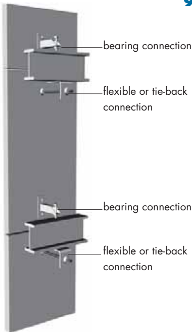
Figure 9-8: Typical push-pull connection for precast panel.
