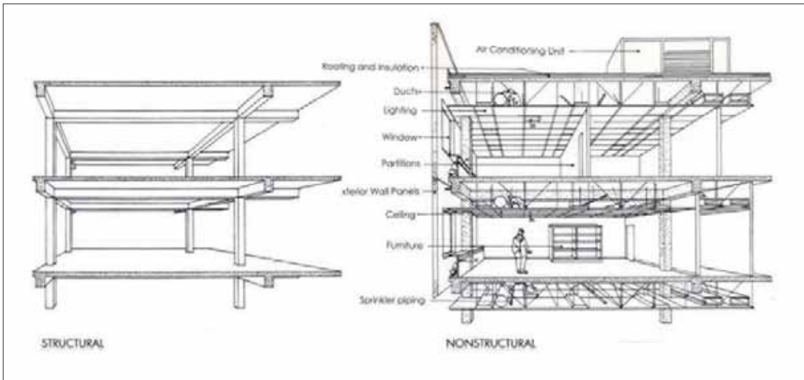
Figure 4-18: Structure (left), nonstructural components and systems (right).
