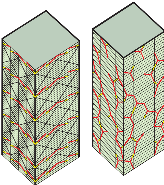
Figure 5-46: Left: 60-story structure with 10 story braced super frame units, restrained by periodic two story moment frame clusters with hydraulic dampers. Right: 48-story moment frames with random offset toggle hydraulic dampers.
