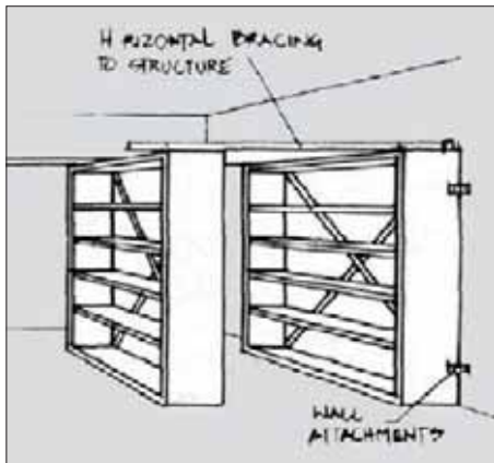
Figure 9-20: Typical layout of bracing for tall shelving.
