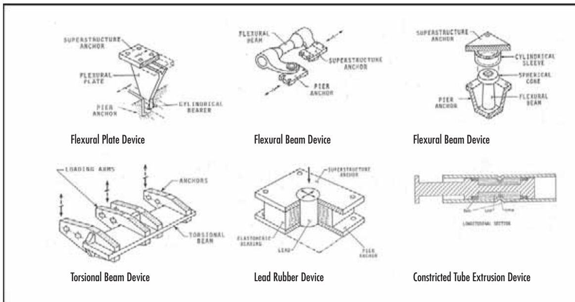
Figure 7-9: A set of energy dissipating devices.
