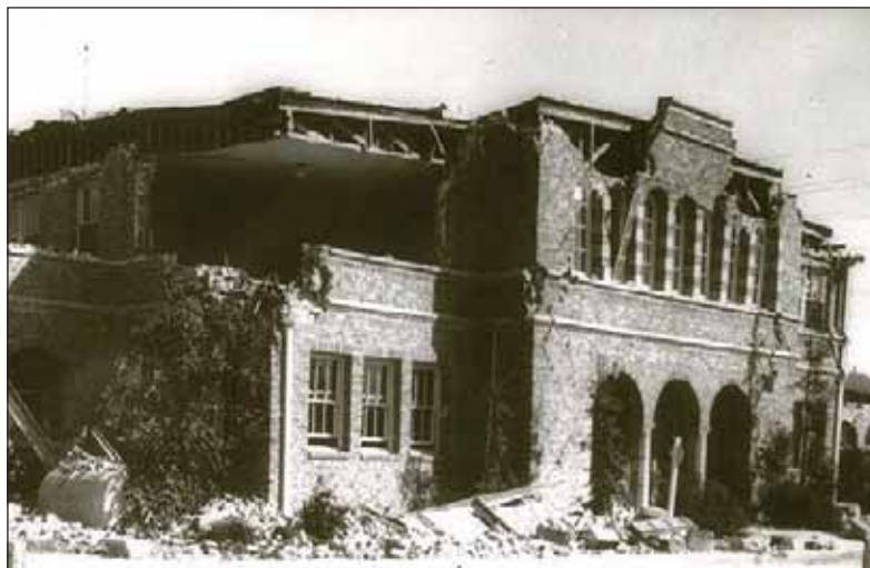
Figure 6-3: Long Beach, 1933, Alexander Hamilton Junior High School.
