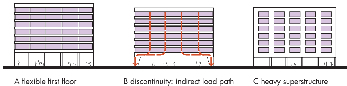
Figure 5-8: Three types of soft first story.
