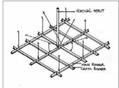
Figure 9-10: Suspended-ceiling seismic bracing.
