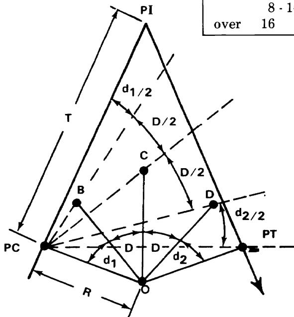
Figure 3-4. Deflection angles
