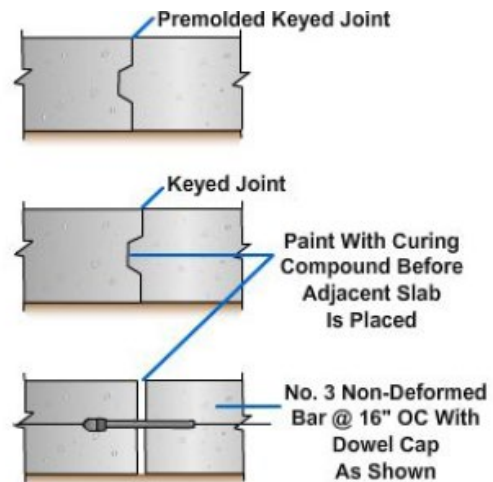
Figure 60 – Types of construction joints.
