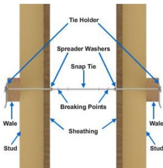
Figure 26 – Snap tie.
