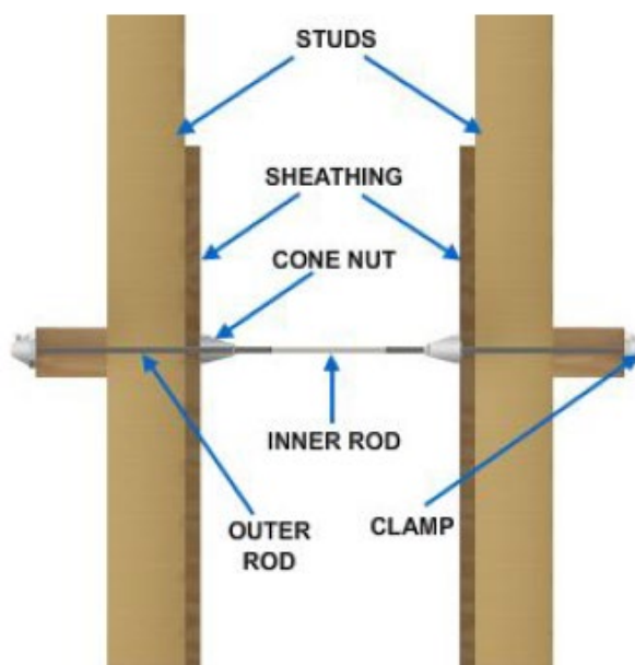
Figure 33 – Tie rod.
