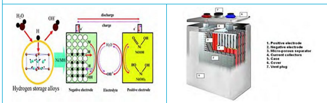
Figure E.3: Chemical and Physical Structures of Nickel–Metal Hybrid Battery
