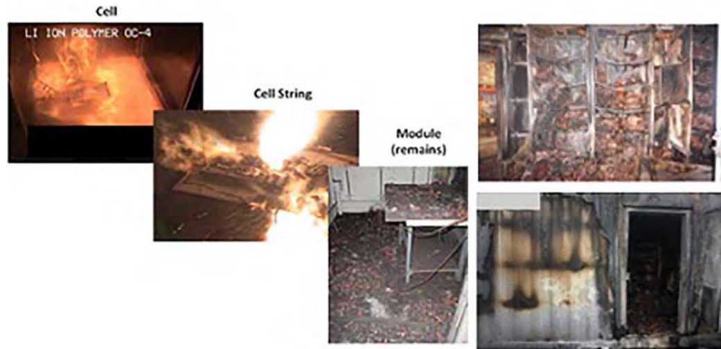
Figure 4.2: Magnified Photos of Fires in Cells, Cell Strings, Modules, and Energy Storage Systems
