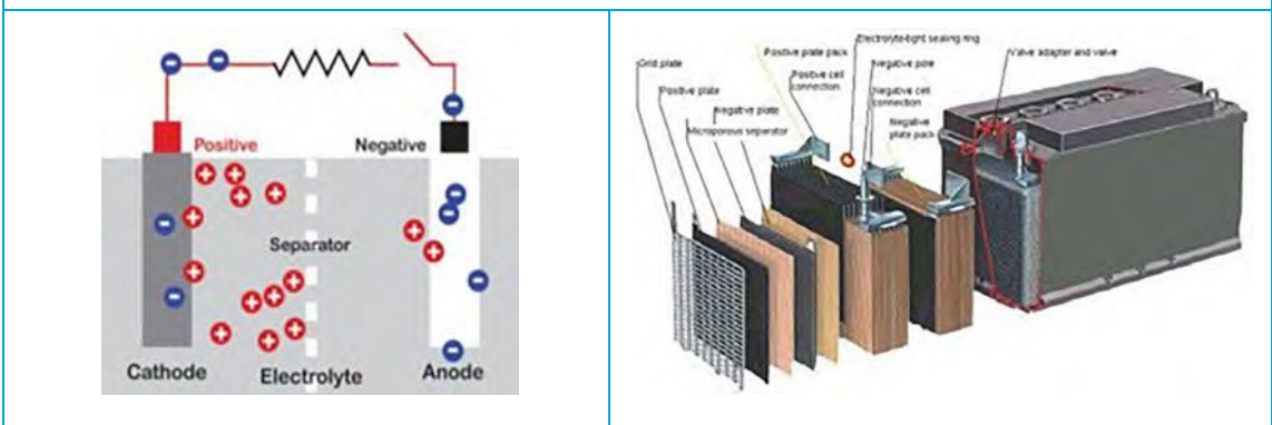
Figure E.1: Lead-Acid Battery Schematic and Physical Structure
