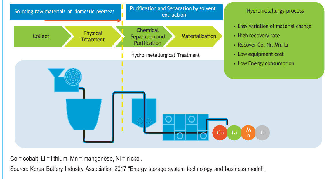
Figure 4.11: Lithium-Ion Battery Recycling Process
