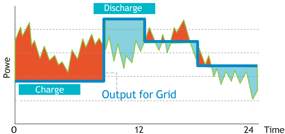
Figure 3.8 Use of Energy Storage Systems for Load Leveling
