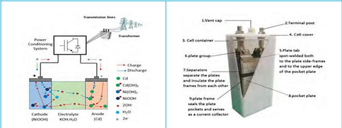
Figure E.2: Chemical and Physical Structures of Nickel-Cadmium Battery
